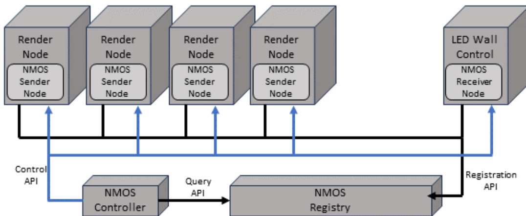
Figure 7: NMOS Control
