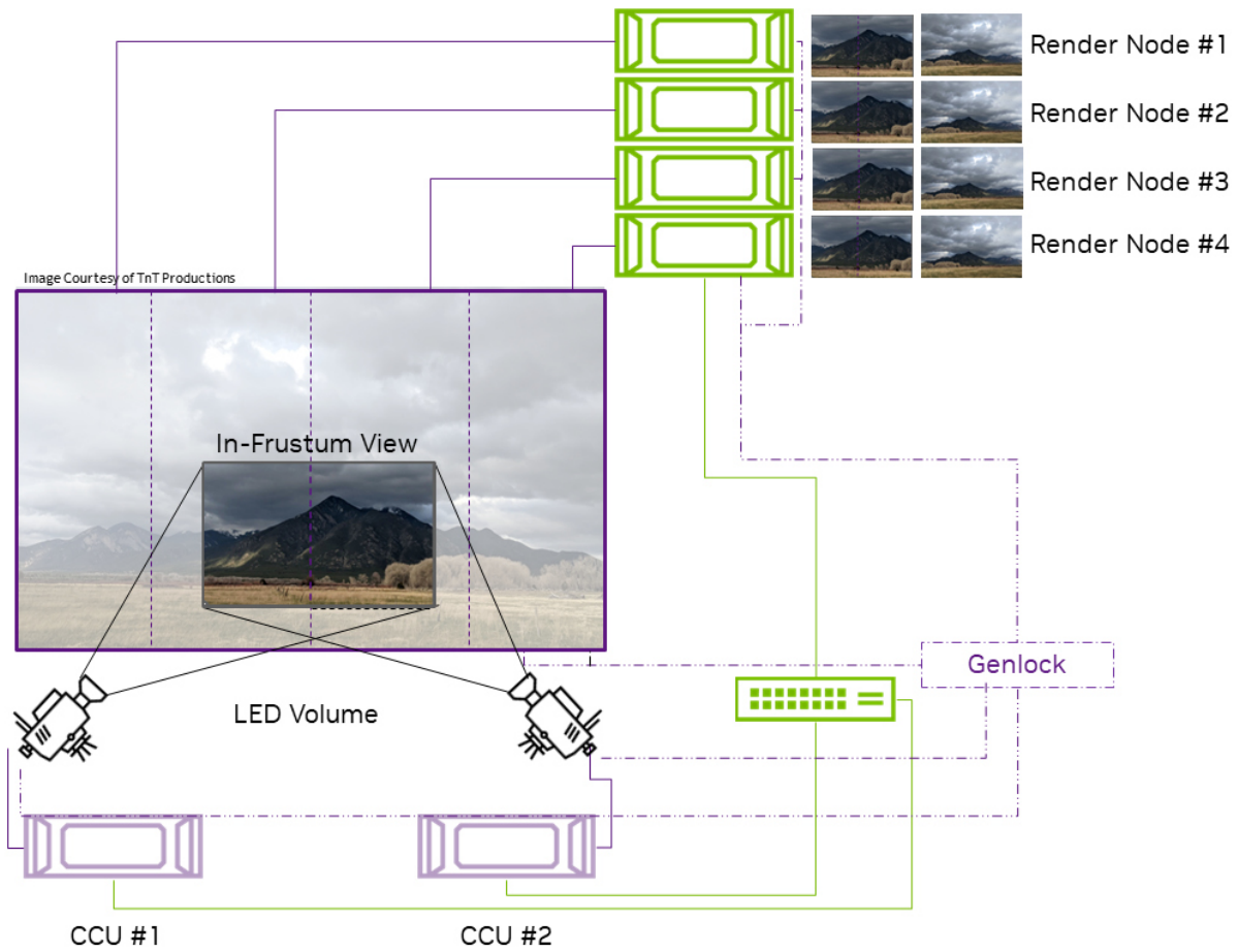
Figure 2: Traditional Virtual Production Stage
